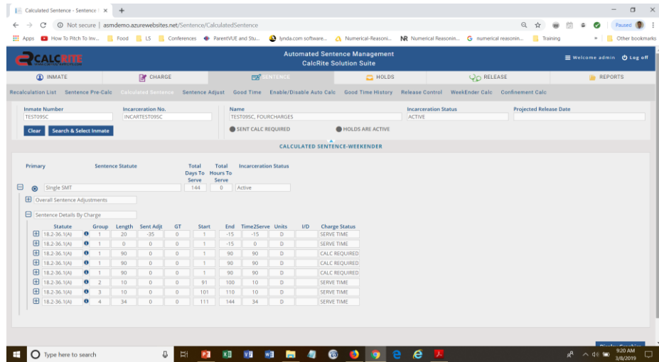
Calculated Sentence
